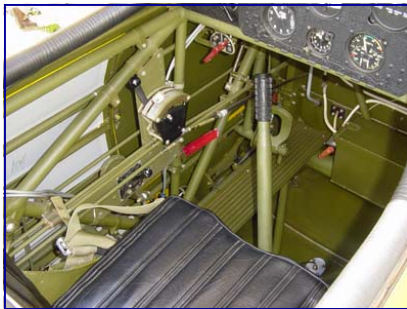
Front Cockpit—Left Side
